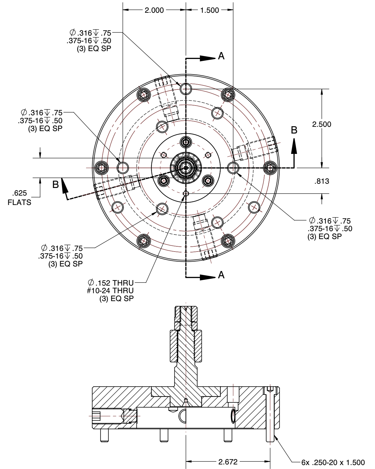
SECTION B-B
