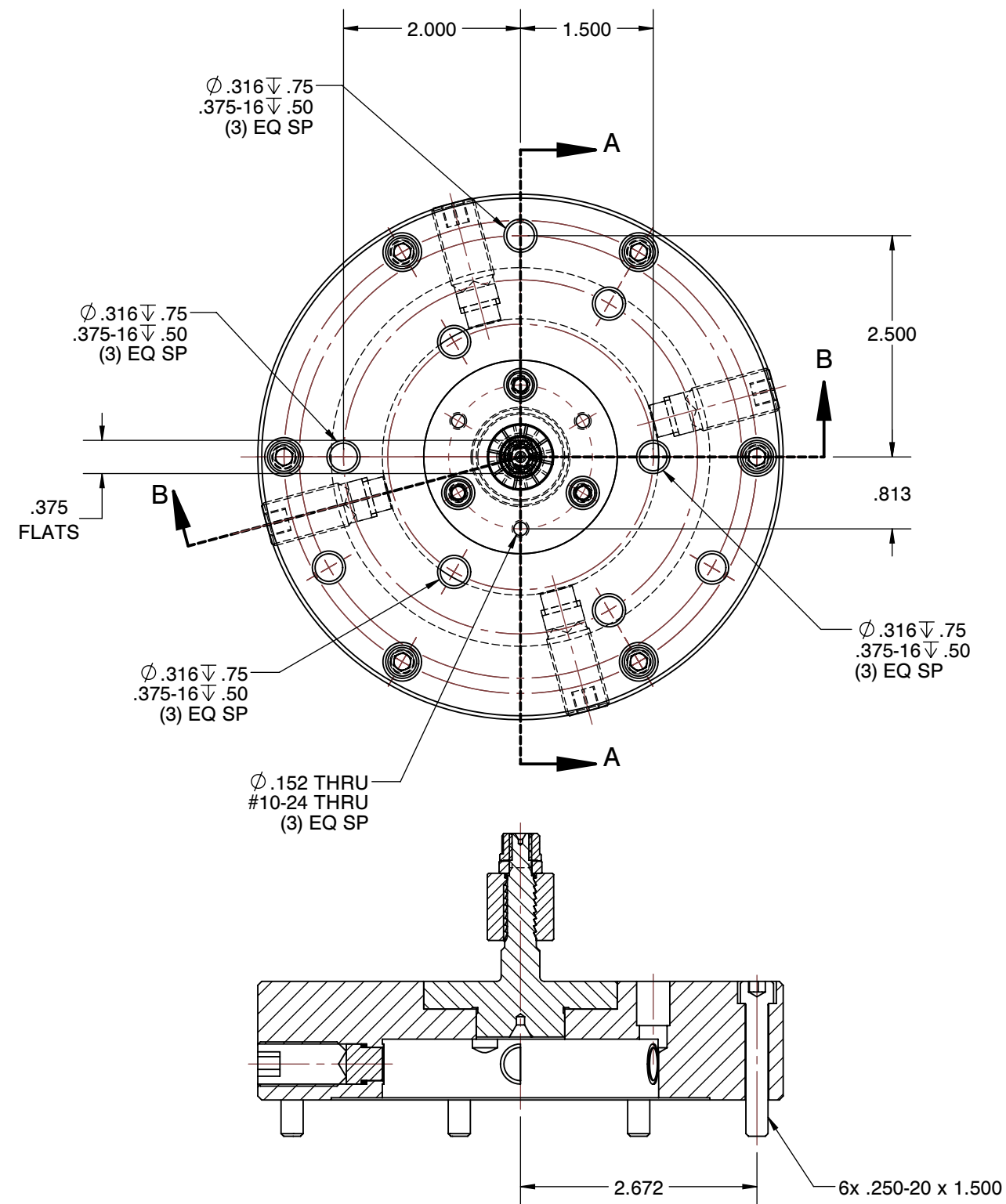
SECTION B-B
