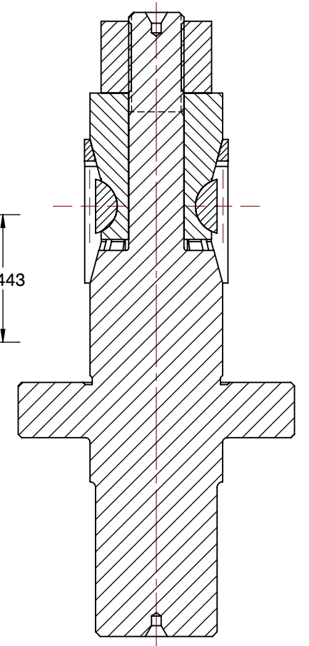
SECTION B-B
