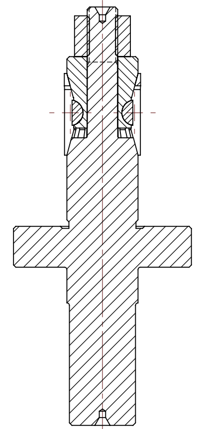
SECTION B-B
