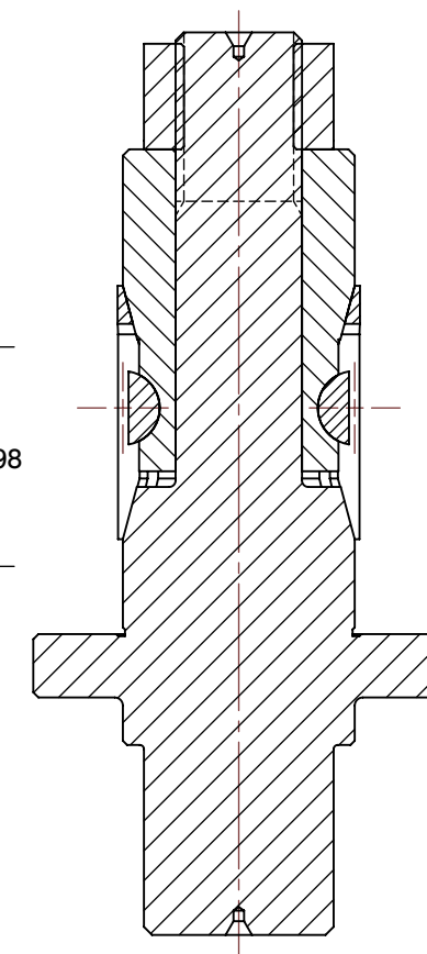
SECTION B-B
