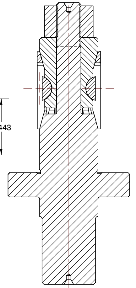
SECTION B-B
