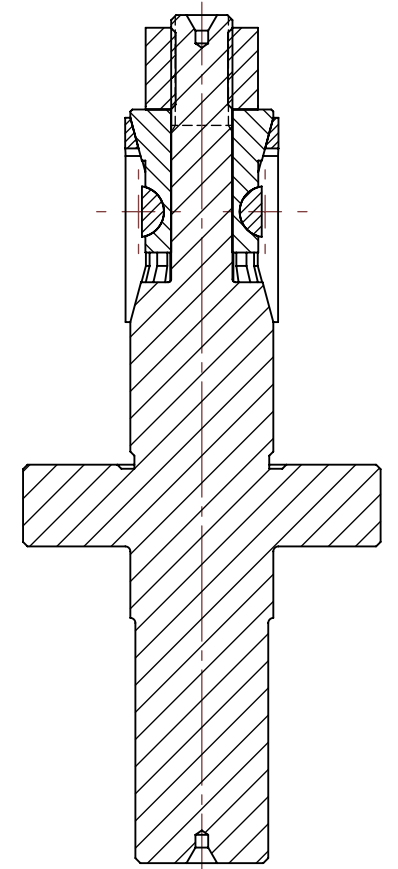
SECTION B-B
