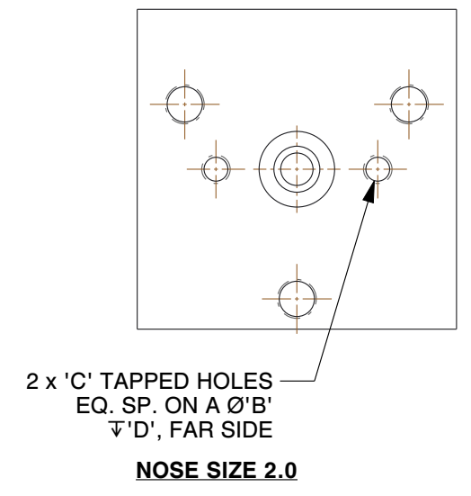
RETAINER ASSEMBLY TAPPED HOLES
