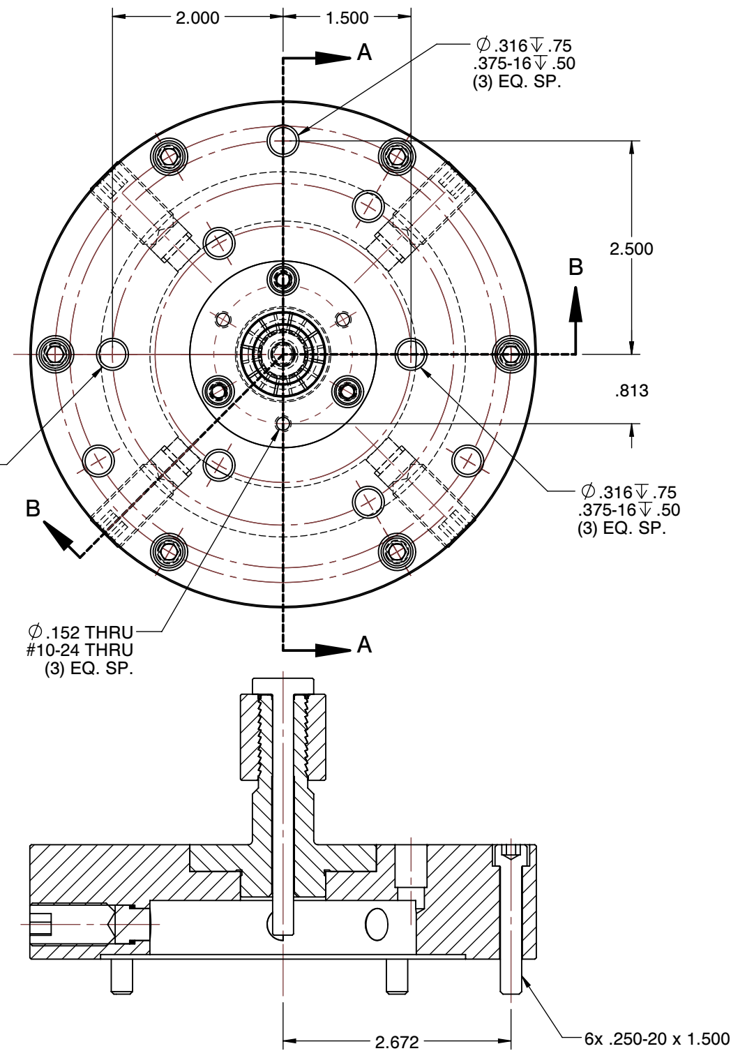
SECTION B-B
