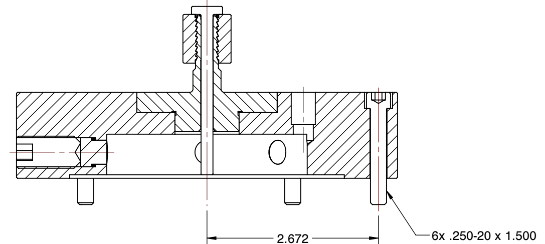
SECTION B-B
